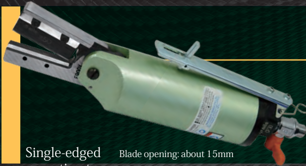
Lever-operated type Blade opening: about 15mm
